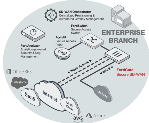
Secure SD-WAN Enterprise Branch Deployment
